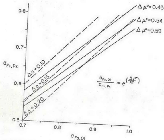
Fig. 4. Solid lines are plots of the function a_{Fs,Ol}/a_{Fs,Px} = \exp(\Delta\mu^\circ/RT) for three values of \Delta\mu^\circ at a temperature of 1173°K (900°C). The ratio of the activity of fayalite in olivine ( a_{Fs,Ol} ) to the activity of ferrosilite in pyroxene ( a_{Fs,Px} ) will fit this equation when the two phases are in equilibrium with high quartz. The dashed lines are plots of \Delta a = a_{Fs,Ol} - a_{Fs,Px} . Values of \Delta a are rather insensitive to the exact values chosen for \Delta\mu^\circ and a_{Fs,Ol} .
